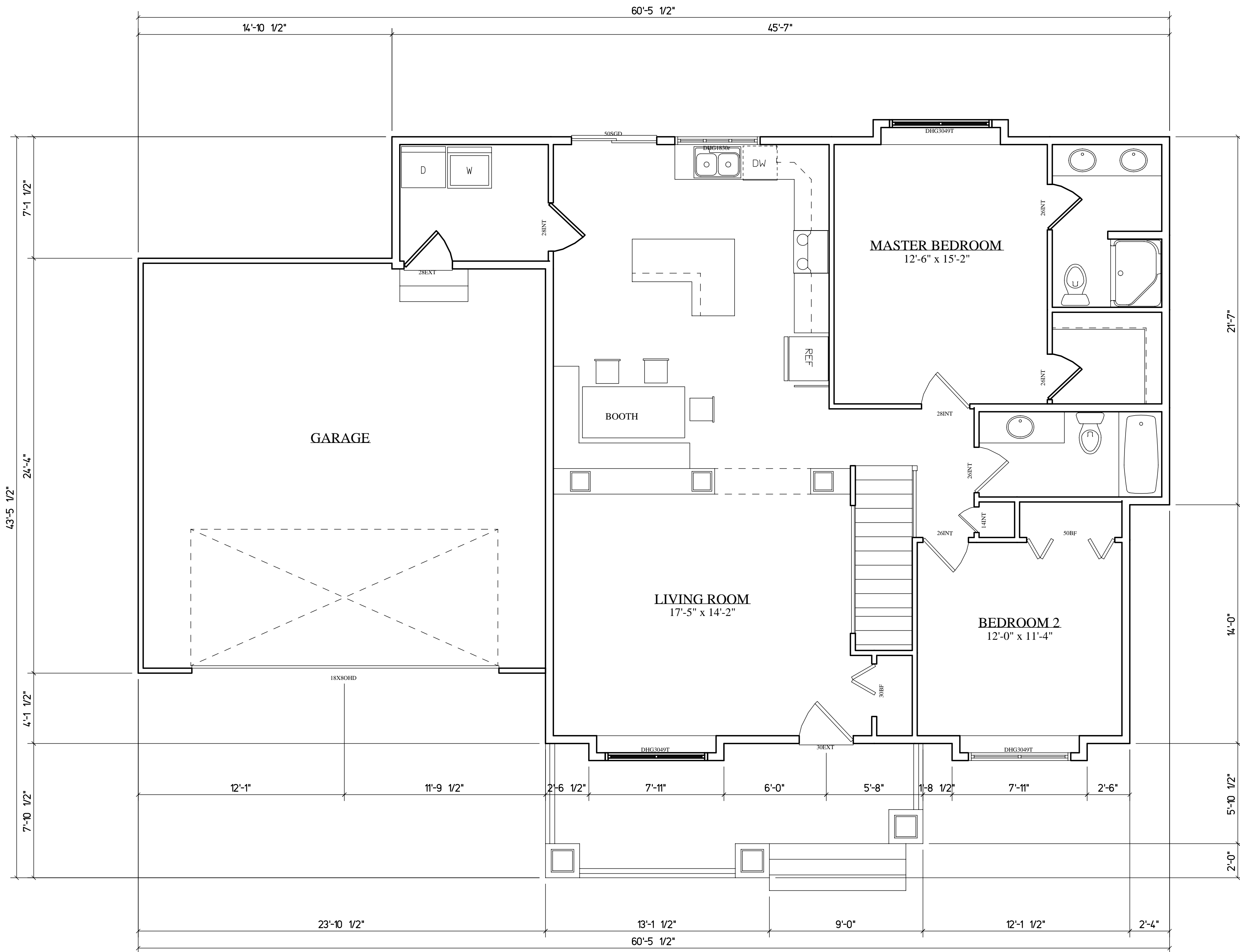
MAIN LEVEL FLOOR PLAN 1,339 SQ. FT.
